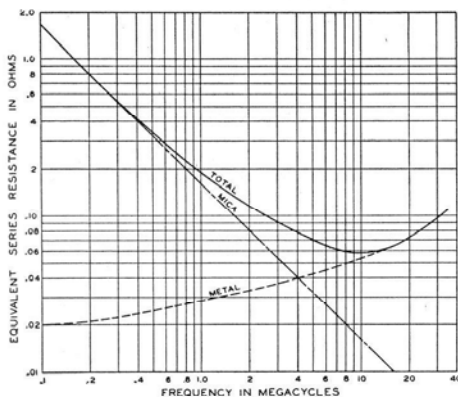
Equivalent-resistance-versus-frequency characteristic of a typical TYPE 505 Condenser
