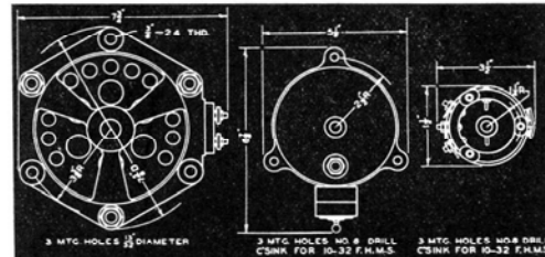
100-K, -L 200-CM, -CU 200-B VARIAC TYPES
