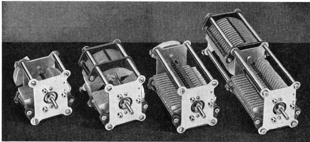
Left to right: TYPE 334-F, TYPE 335-Z, TYPE 334-R, and TYPE 334-Z
